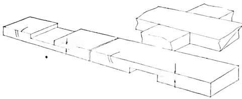
FIG. 243. CROSS-LAP JOINT.
